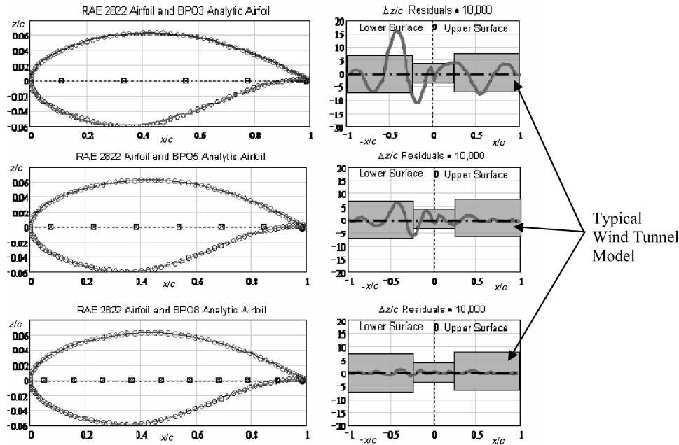
Fig. 10 RAE2822 airfoil shape convergence study.
