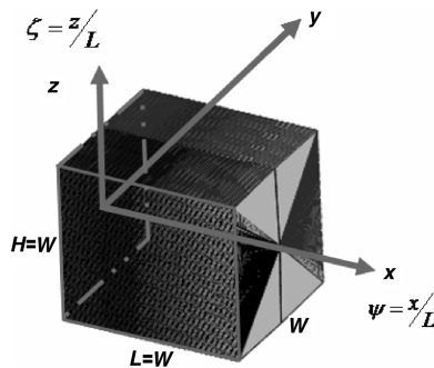
Fig. 23 Definitions of cross section shape and distribution.
