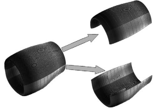
Fig. 32 Total nacelle external shape and inlet geometry definition (15 variables).
