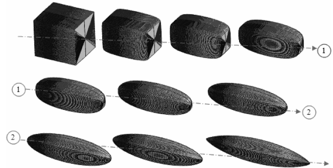
Fig. 25 Three variable transformation of a cube into a Sears–Haack body.
