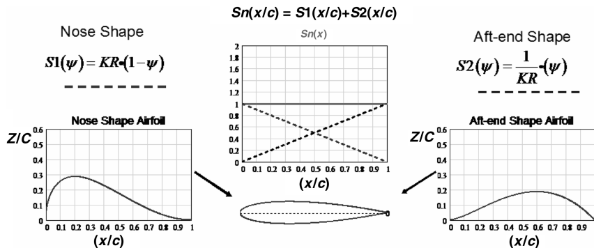
Fig. 5 Airfoil decomposition into component shapes or basis functions.
